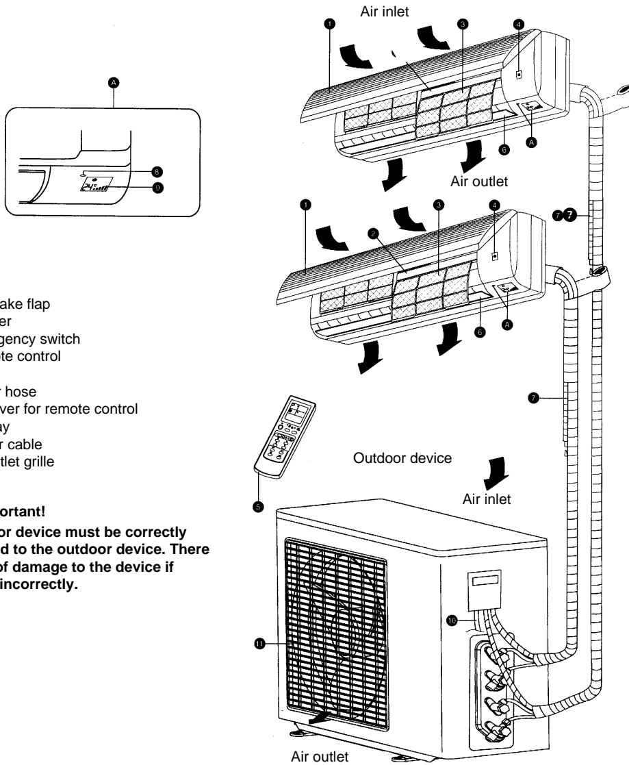
Indoor device
